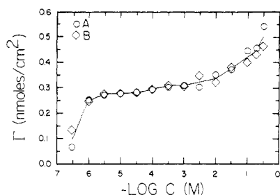
Figure 29. Packing density, \Gamma , of HQ/BQ at Pt(111). (A) \Gamma , based upon I_C/I_{Pt} , eq 34; (B) \Gamma , based upon I_{Pt}/I_{Pt} , eq 35. Experimental conditions: supporting electrolyte, 10 mM KF adjusted to pH 4 with HF; electrode potential, 0.2 V vs Ag/AgCl (1 M KCl) reference; temperature, 23 \pm 1^\circ\text{C} . Reprinted with permission from ref 44. Copyright 1988 American Chemical Society.
