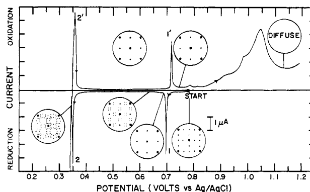
Figure 9. Cyclic voltammogram and LEED patterns for deposition of Ag at the Pt(100) Pt(100)[ c(\sqrt{2} \times \sqrt{8}) ]R45°-I adlattice. Experimental conditions: 1.0 mM \text{Ag}^+ in 1 M \text{HClO}_4 ; scan rate, 2 mV/s. Reprinted with permission from ref 29. Copyright 1984 American Chemical Society.
