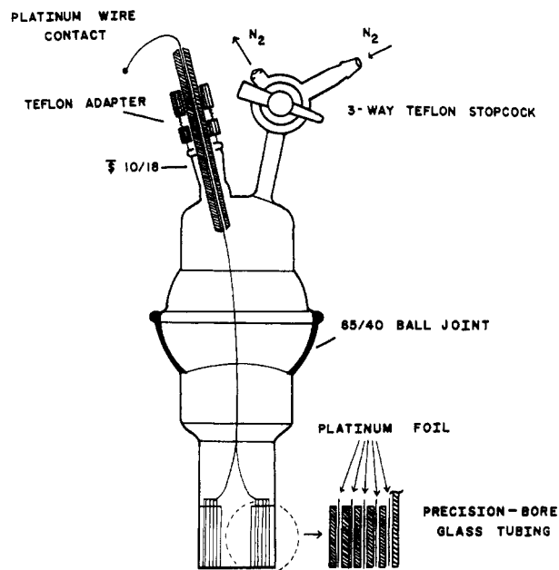
Figure 23. Large-area thin-layer electrode. Area = 168 cm 2 ; volume = 0.90 cm 3 . Reprinted with permission from ref 73. Copyright 1986 American Chemical Society.
