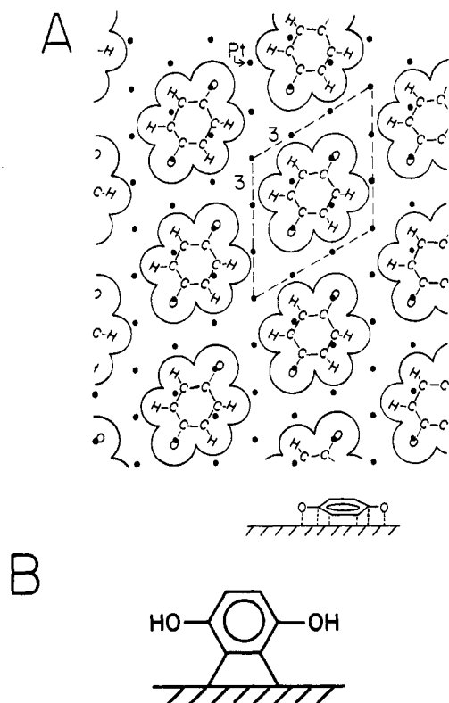
Figure 31. Structure of BQ/HQ adsorbed at Pt(111). (A) Pt(111)(3×3)-BQ/HQ, \theta = 1/9 ( \Gamma = 0.276 \text{ nmol/cm}^2 ); (B) Vertical orientation of adsorbed HQ (2,3- \eta^2 ). Reprinted with permission from ref 44. Copyright 1988 American Chemical Society.
