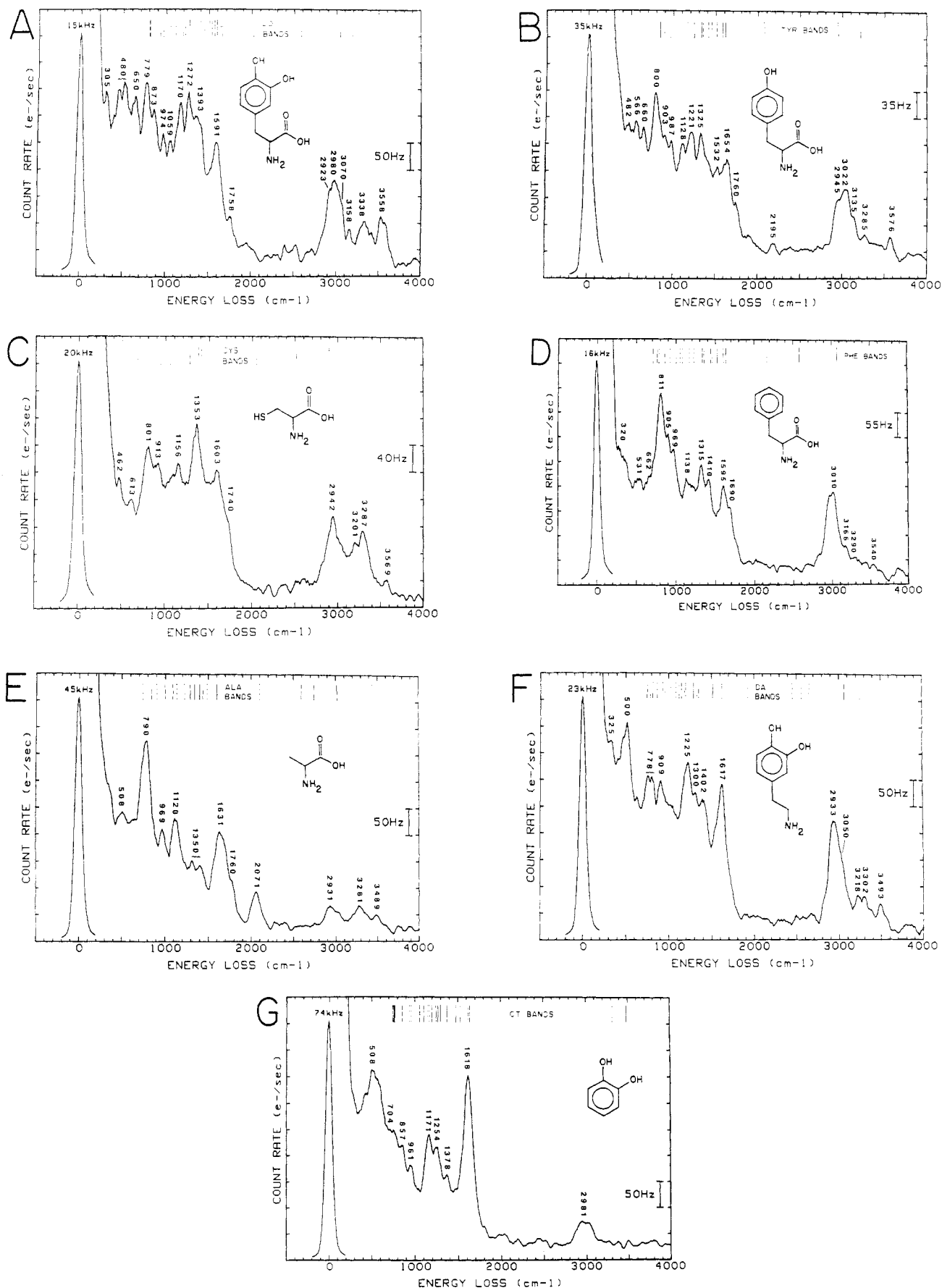
Figure 34. EELS spectra of adsorbed amino acids and related compounds at Pt(111). (A) L-Dopa, (B) L-tyrosine, (C) L-cysteine, (D) L-phenylalanine, (E) L-alanine, (F) dopamine, (G) catechol. Experimental conditions: adsorbate concentrations (mM) were LD (5.0), Tyr (1.0), Cys (0.5), Phe (1.0), Ala (1.0), DA (1.0), CT (1.0); other conditions were as in Figure 30. Reprinted with permission from ref 47. Copyright 1988 American Chemical Society.
