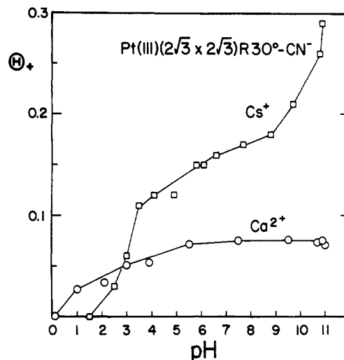
Figure 5. Cation packing density vs pH at Pt(111) (2\sqrt{3} \times 2\sqrt{3})\text{R}30^\circ\text{-CN}^- . Experimental conditions: The CN layer was immersed into 0.1 mM \text{Cs}^+ or \text{Ca}^{2+} ; the pH was adjusted by means of HCl, CsOH, or Ca(OH); the electrode potential was 0.1 V (Ag/AgCl/1 M KCl reference). Reprinted with permission from ref 21. Copyright 1985 American Chemical Society.
