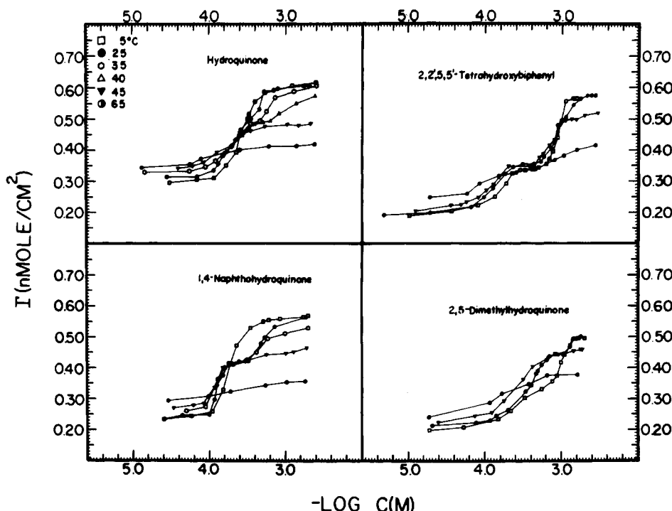
Figure 17. Packing density, \Gamma (nmol/cm 2 ), vs adsorbate concentration at various temperatures. Experimental conditions: polycrystalline Pt thin-layer electrode; 1 M HClO 4 electrolyte. Reprinted with permission from ref 53. Copyright 1983 American Chemical Society.
