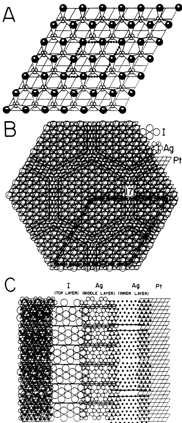
Figure 8. Surface structures of Ag electrodeposited at iodine-pretreated Pt(111). (A) Pt(111)(3×3)-Ag,I, \theta_{\text{Ag}} = \theta_{\text{I}} = 4/9 ; (B) Pt(111)( \sqrt{3} \times \sqrt{3} )R30°-Ag,I with 17-unit domains, \theta_{\text{Ag}} = 2/3 , \theta_{\text{I}} = 1/3 ; (C) Pt(111)( \sqrt{3} \times \sqrt{3} )R30°-Ag,I with 11-unit (middle layer) and 17-unit (lower layer) domains, \theta_{\text{Ag}} = 5/3 , \theta_{\text{I}} = 1/3 . Reprinted with permission from ref 16 and 23. Copyright 1983 Elsevier.
