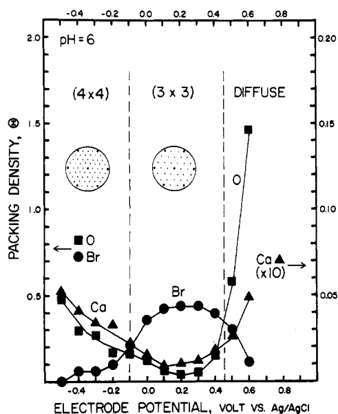
Figure 2. Adsorption profiles of Br, Ca, and O from 0.05 mM \text{CaBr}_2 (pH 6) at Pt(111) as a function of electrode potential (Ag/AgCl/1 M KCl reference). Reprinted with permission from ref 9. Copyright 1986 American Chemical Society.
