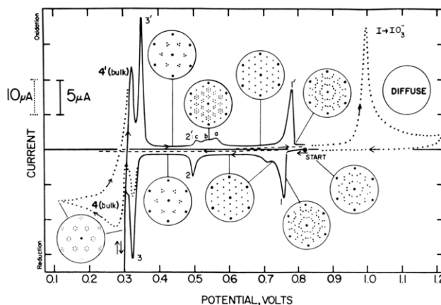
Figure 7. Cyclic voltammogram and LEED patterns. Experimental conditions: 0.1 mM Ag + in 1 M HClO 4 at the Pt(111)-( \sqrt{7}\times\sqrt{7} )R19°-I surface; scan rate, 2 mV/s. Reprinted with permission from ref 22. Copyright 1983 Elsevier Sequoia.
