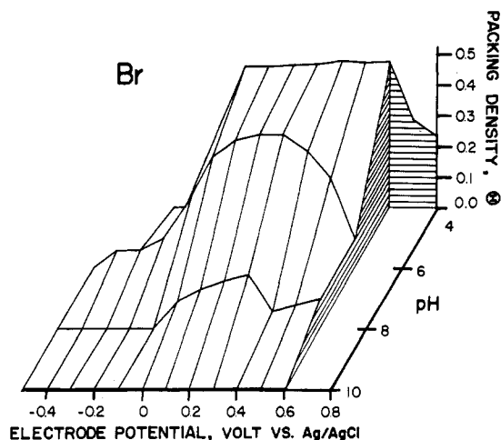
Figure 1. Isometric projection of the adsorption profiles of Br (0.05 mM \text{CaBr}_2 ) at Pt(111). Reprinted with permission from ref 9. Copyright 1986 American Chemical Society.
