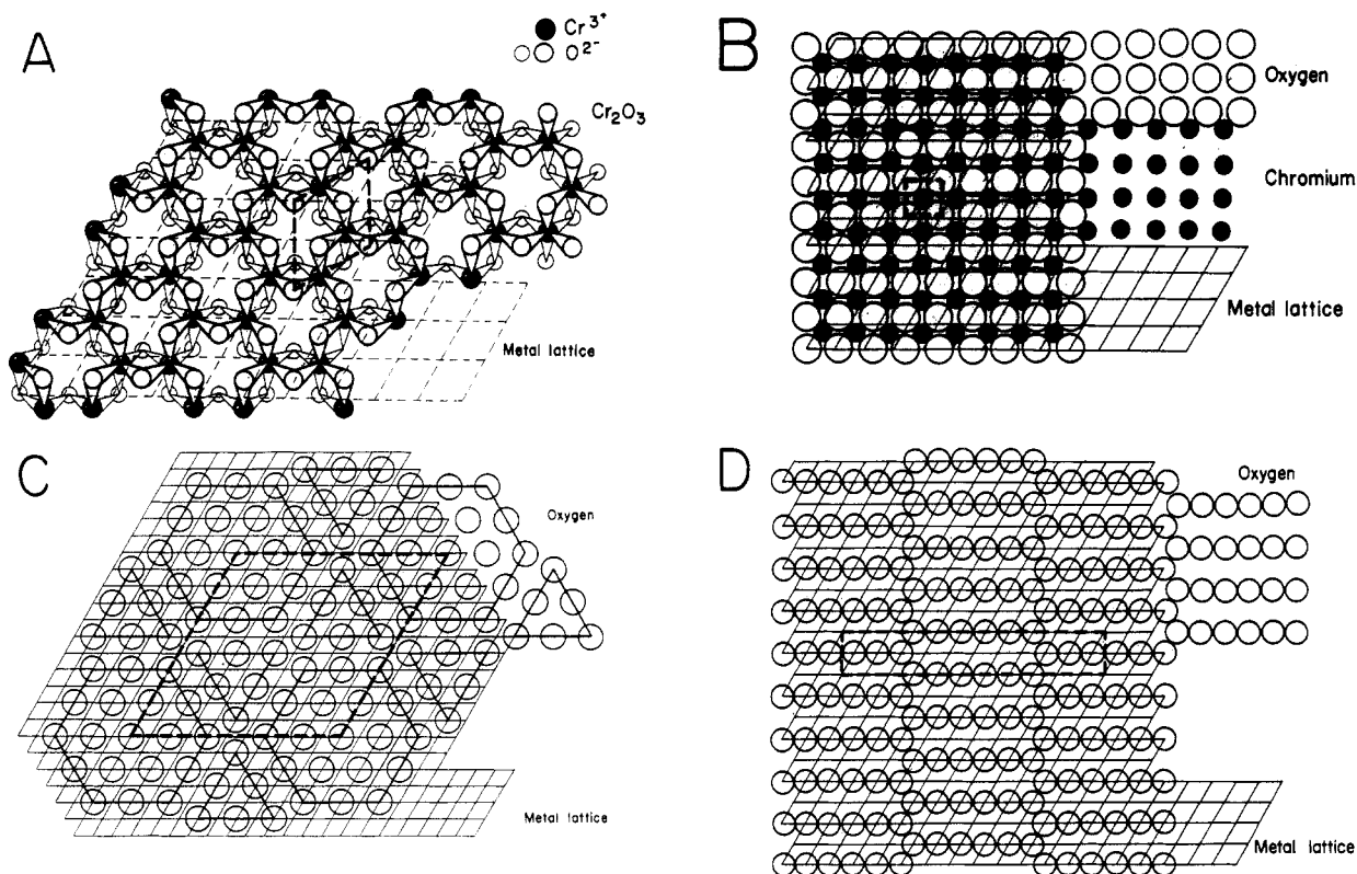
Figure 13. Surface structures at FeCrNi(111). (A) (001) plane of the \text{Cr}_2\text{O}_3 structure situated on the alloy substrate as experimentally determined. (For clarity, only a few layers of the oxide are shown.), (B) Square \text{CrO} structure, (C) Growth phase structure ( 11 \times 11 ), (D) Alternative growth phase structure ( 11 \times \sqrt{3} ). Reprinted with permission from ref 38. Copyright 1985 American Chemical Society.
